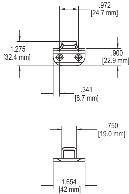
FIG. 3 18.16 SASH LIFT
