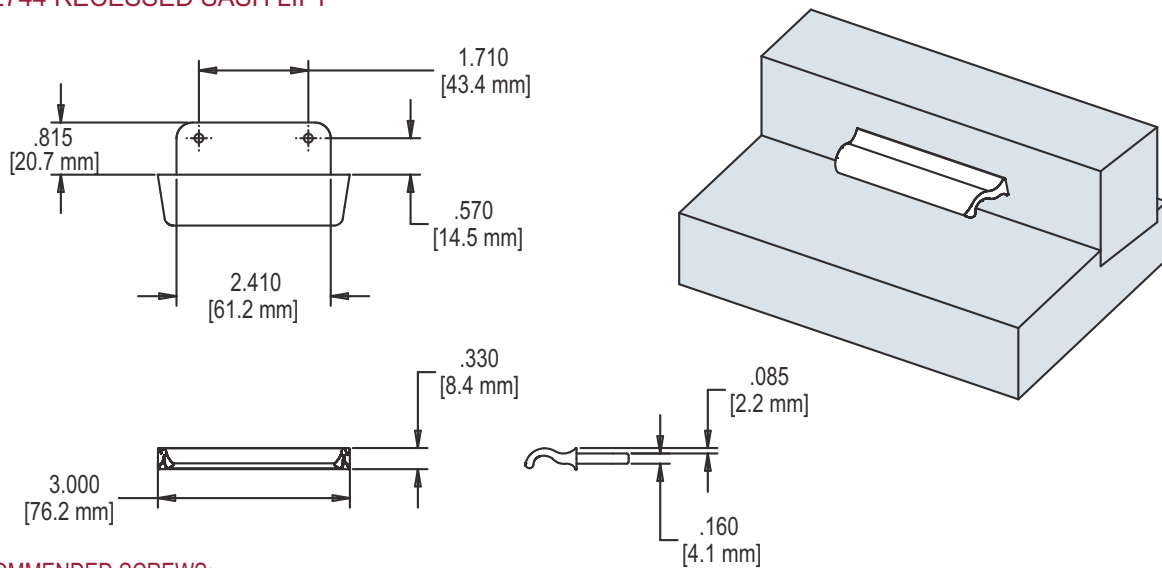
FIG. 6 32744 RECESSED SASH LIFT
