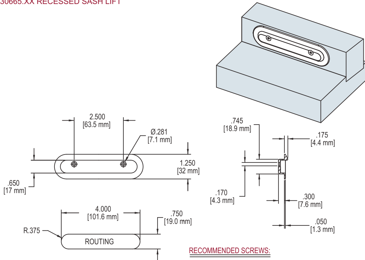
FIG. 5 30665.XX RECESSED SASH LIFT
