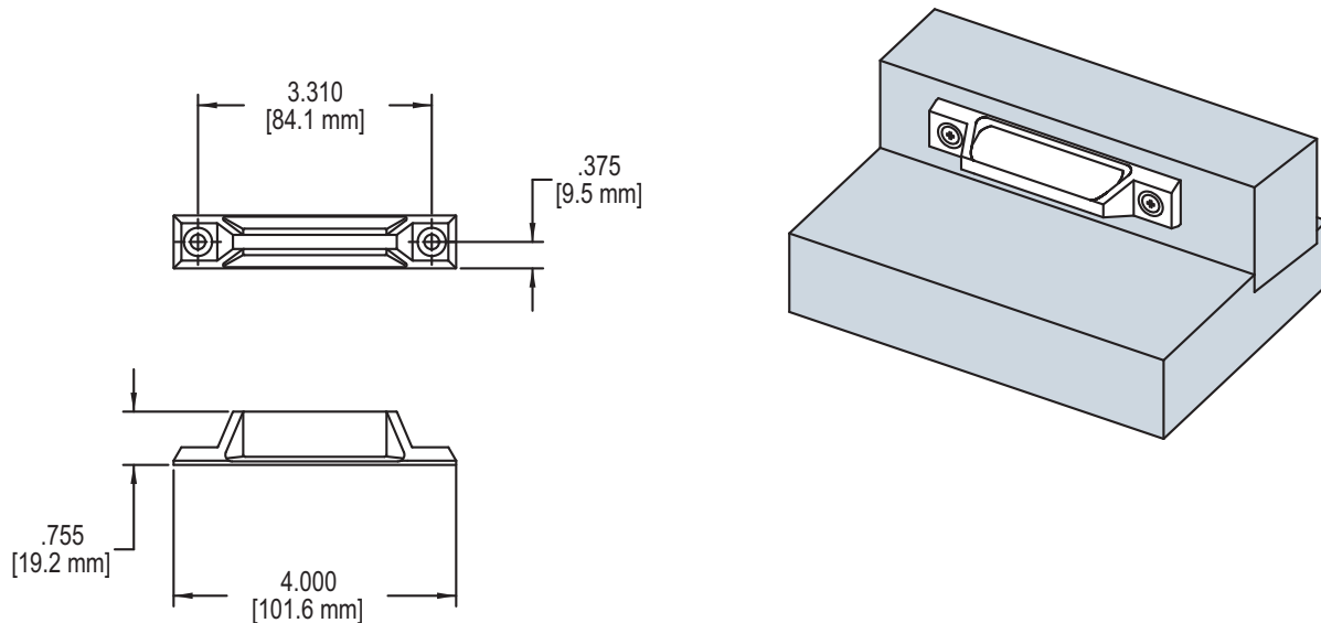
FIG. 1 18.10 SASH LIFT
